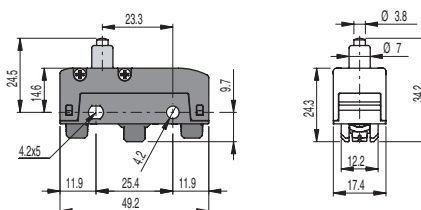
MK V11D03 1S+1Ö PC 0,5 mm FS 4 N OC 2 mm FR 3 N CD 0,05 mm
